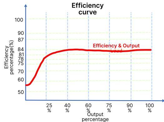
Figure 5: Efficiency Vs Output Load (Nominal Voltage Input)
