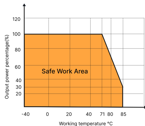
Figure 4: Temperature Derating Curve DCK78U24-0.3A(L), (Vin > 60V)
