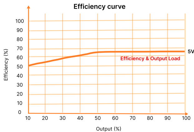
Figure 5: Efficiency Vs Output Load (Nominal Voltage Input)
