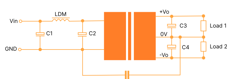
Figure 2: EMC Typical Recommended Circuits
