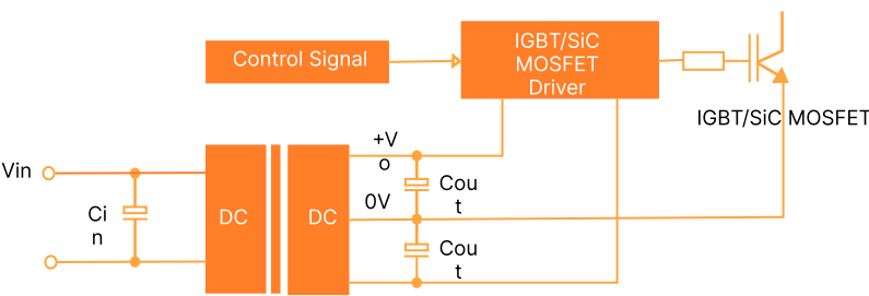
Figure 1: Application circuit
