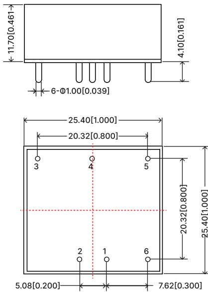
Figure 7: Overall dimensions
