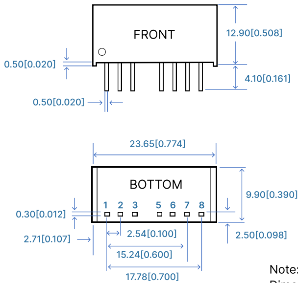
Figure 7: Overall dimensions
