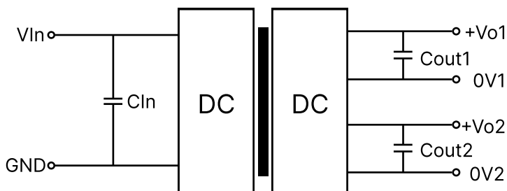
Figure 1: Application circuit
