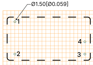
Note: The grid distance is 2.54mm*2.54mm
