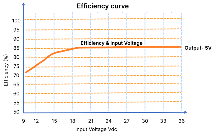
Figure 5: Efficiency Vs Input Voltage (100% Load)
