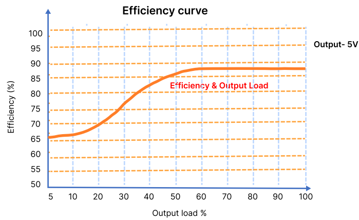
Figure 5: Efficiency Vs Output Load (Nominal Voltage Input)
