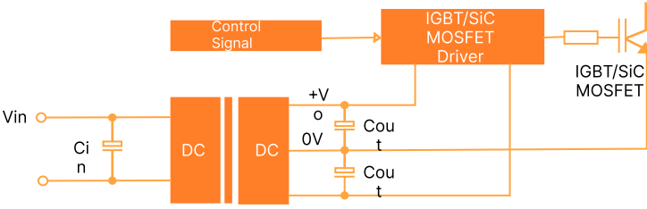
Figure 1: Application circuit
