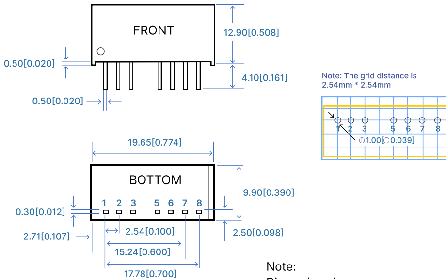
Figure 7: Overall dimensions
