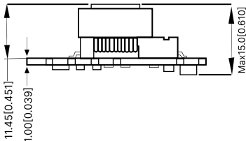
Figure 7: Overall dimensions
