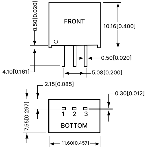
Figure 7: Overall dimensions
