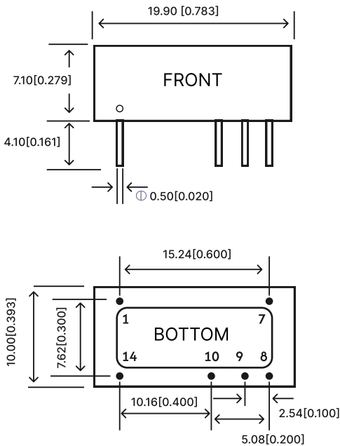
Figure 7: Overall dimensions
