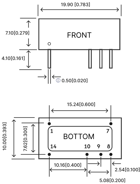
Figure 7: Overall dimensions
