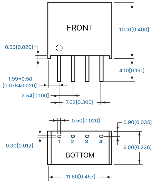
Figure 7: Overall dimensions
