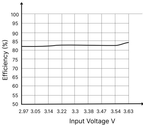
Figure 6: Efficiency Vs Input Voltage
