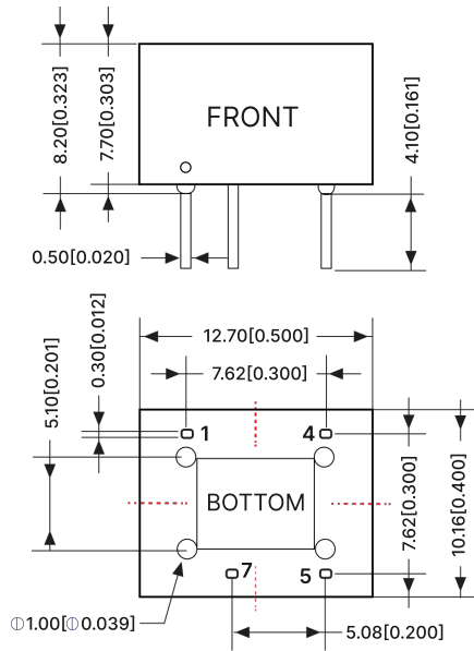
Figure 7: Overall dimensions
