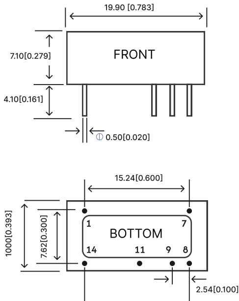
Figure 7: Overall dimensions
