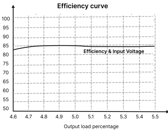
Figure 6: Efficiency Vs Input Voltage (100% Load)
