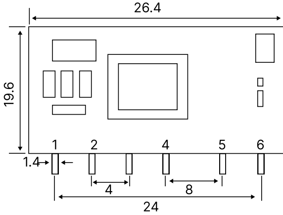
Figure 7: Overall dimensions
